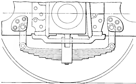
Fig. 3—Test Spring With Non-Adjustable Spring Link
